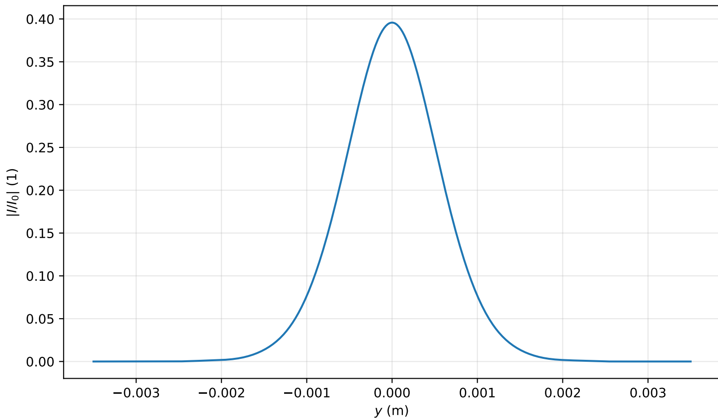
Intensity profile I(x=0, y, z=3.503)/I_0 , P_{in}=0.4P_{cr} , artificial time
